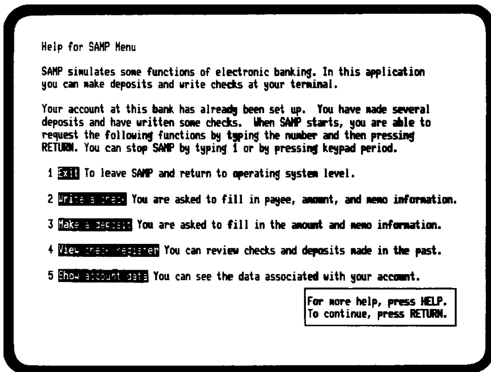
Figure 3.8. Menu Help Form
