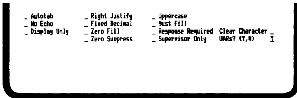
Figure 7.7. Assigning User Action Routines
