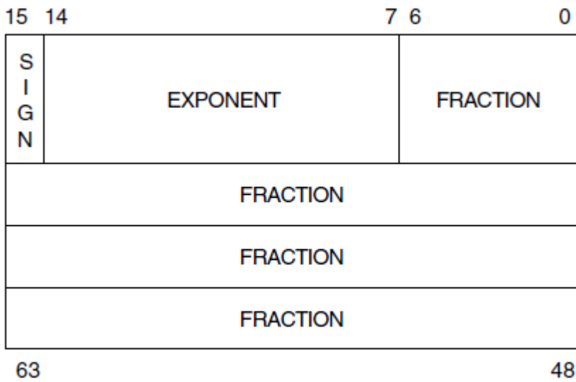
Figure 17.6. Double-Precision Real Number Format
