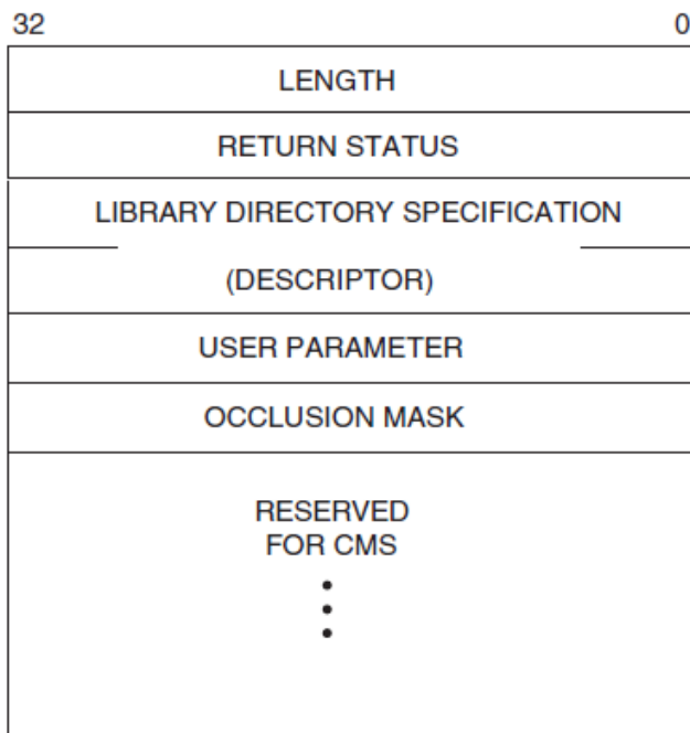
Figure 1.1. A CMS Library Data Block
