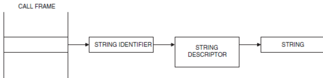
Figure 1.2. A String Identifier
