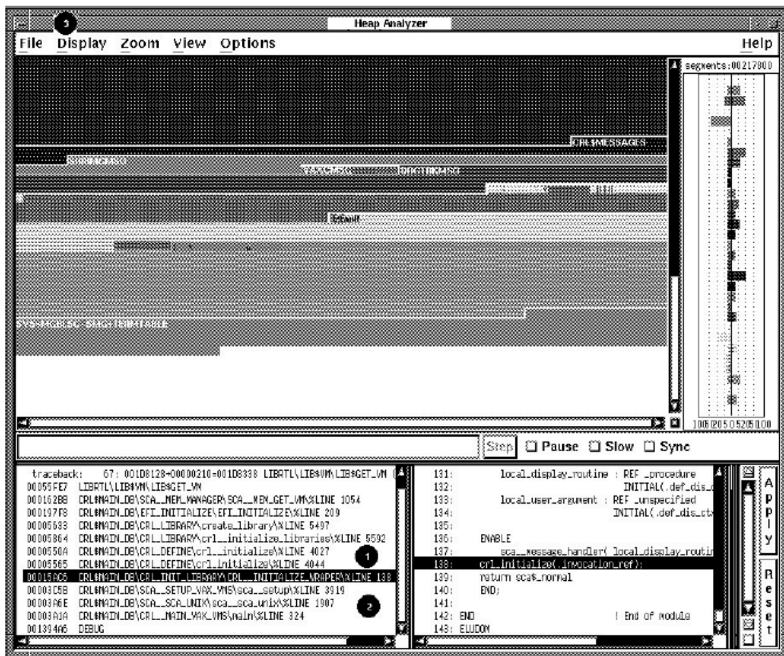
Figure 12.7. Heap Analyzer Information and Source Windows
